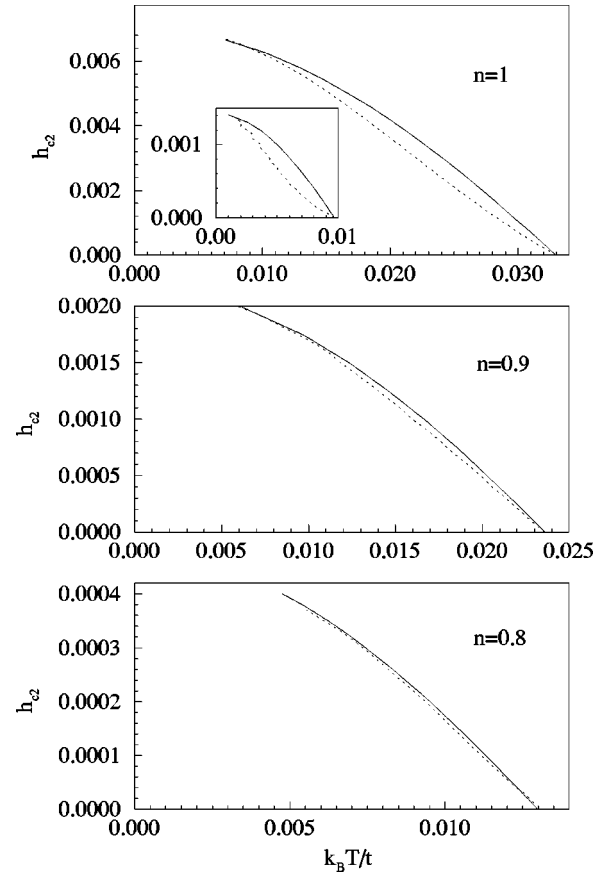
FIG. 5. The upper critical field obtained for the on-site pairing with t'=0 (dashed lines) fitted to the results obtained for the two-dimensional version of the Helfand–Werthamer approach to the Gor’kov equations (continuous lines). We have chosen the pairing potential V=t , for different values of the occupation number n , indicated in the figures. The inset shows results obtained for V=0.7t and n=1 .
