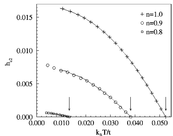
FIG. 3. The same as in Fig. 2, but for anisotropic pairing. The cross, circle, and square marks indicate results obtained on the 120 \times 120 cluster, whereas the solid lines correspond to the 150 \times 150 cluster. The arrows show the d -wave superconducting transition temperature for an infinite system calculated from the BCS gap equation in the absence of magnetic field. Here, V = 0.3t and t' = 0 have been assumed.
